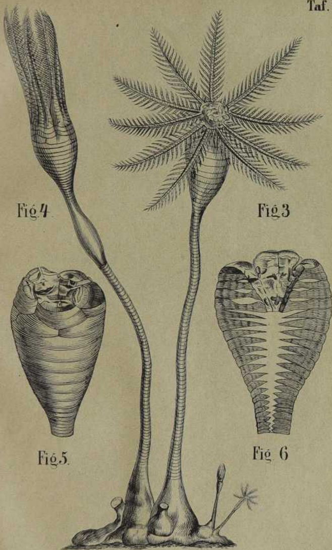
Apiocrinites rotundus.
